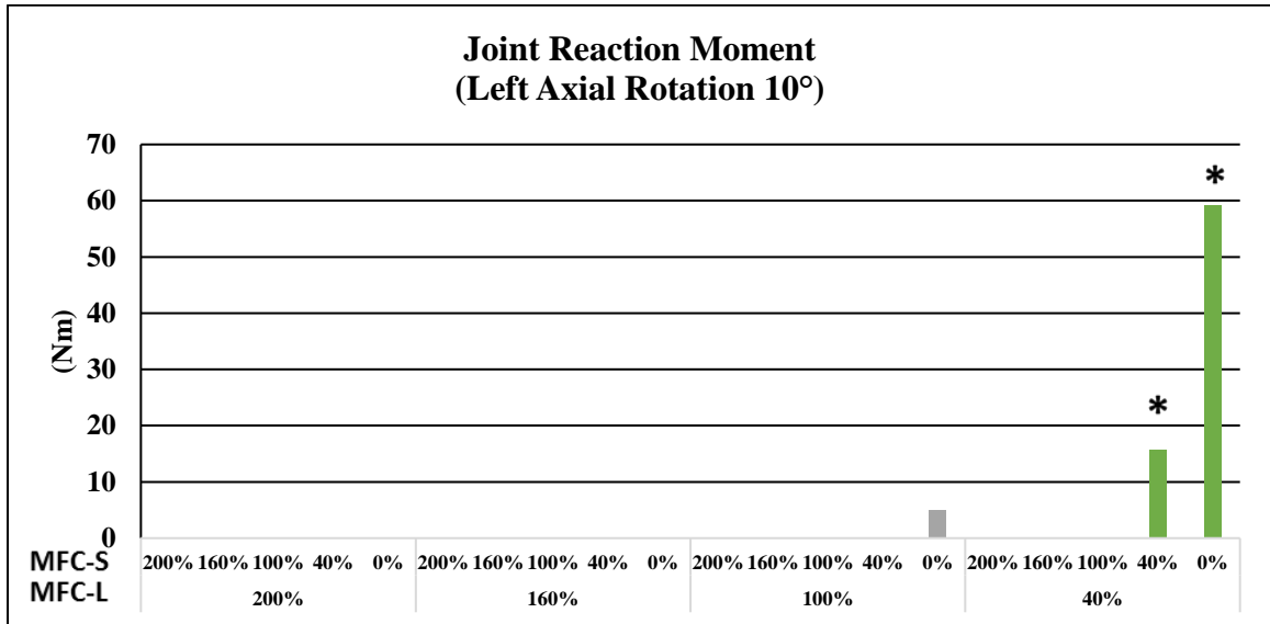
Figure 4-12 A prediction of total joint reaction moments (JRMs) in MFC variation of SIMs and long muscles for left axial rotation 10°. (* Trunk sway > 10, buckling case)
